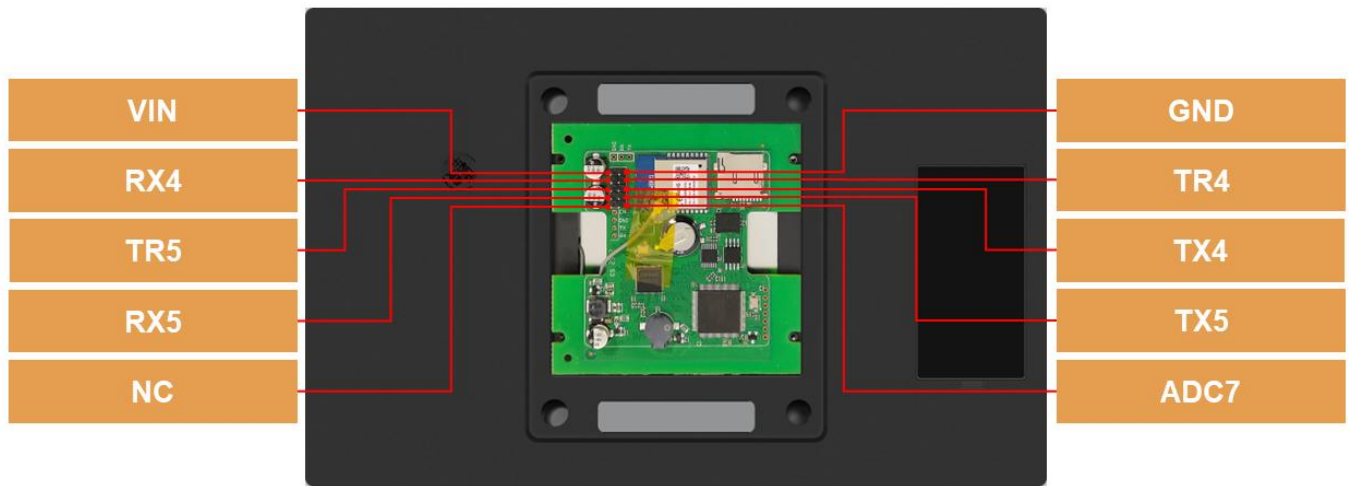
对插接口引脚定义 Board-to-Board connector pinout
