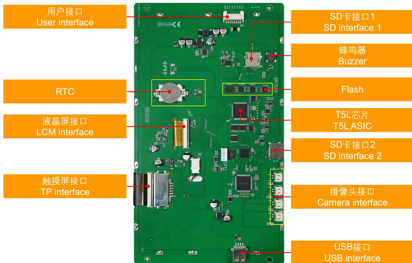
硬件接口图 Hardware interface
