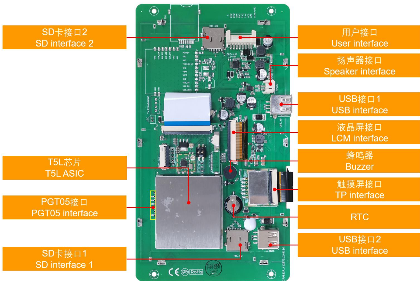
硬件接口图 Hardware interface
