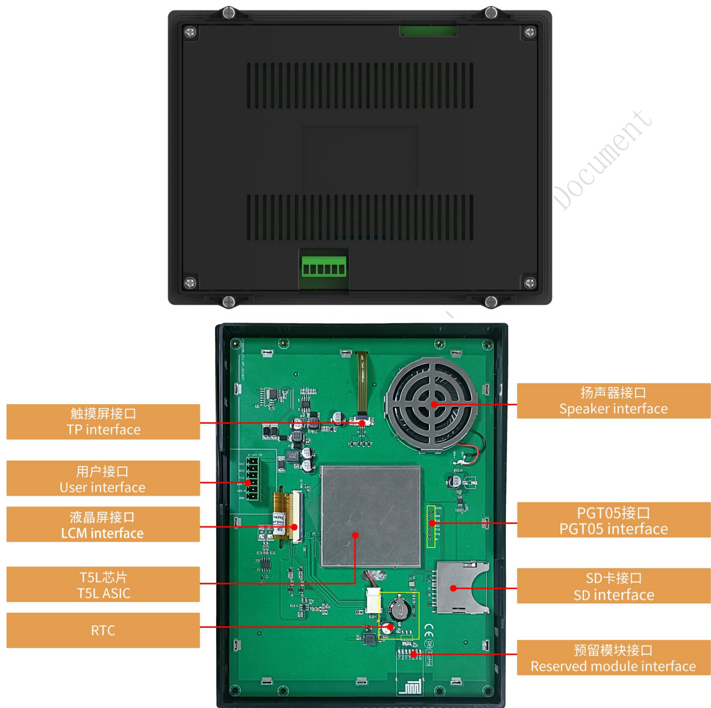
硬件接口图 Hardware interface
