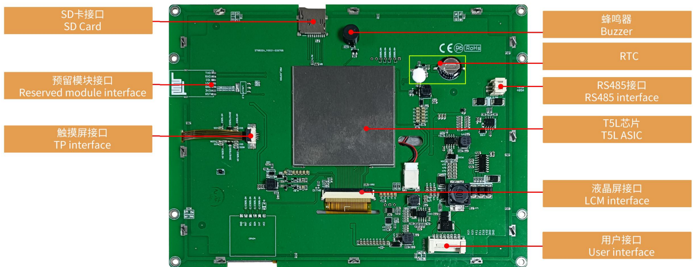
硬件接口图 Hardware interface
