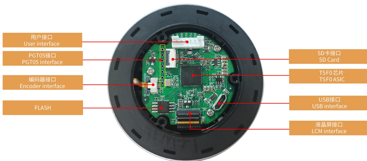
硬件接口图 Hardware interface diagram
