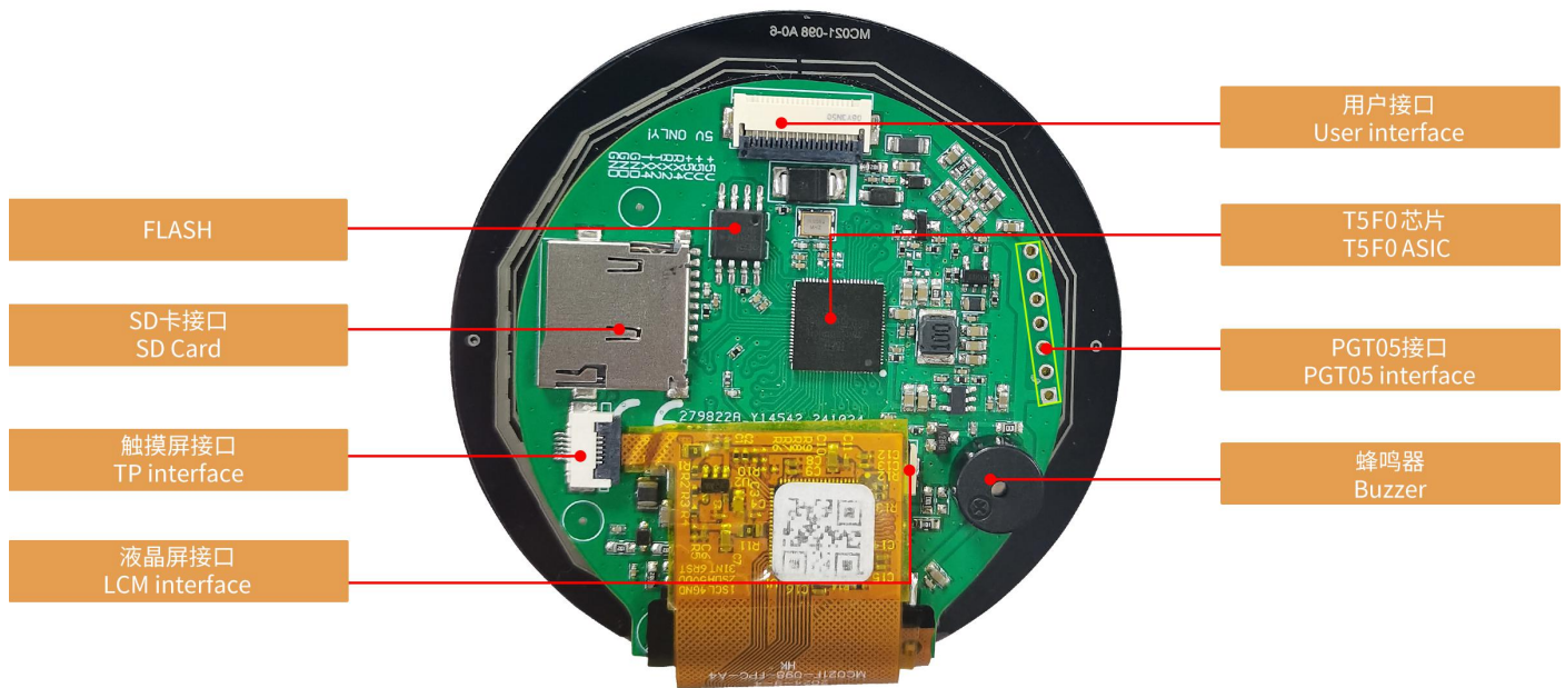
硬件接口图 Hardware interface diagram
