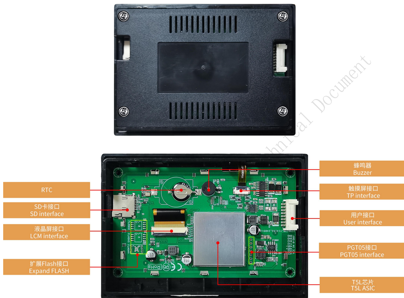
硬件接口图 Hardware interface diagram
