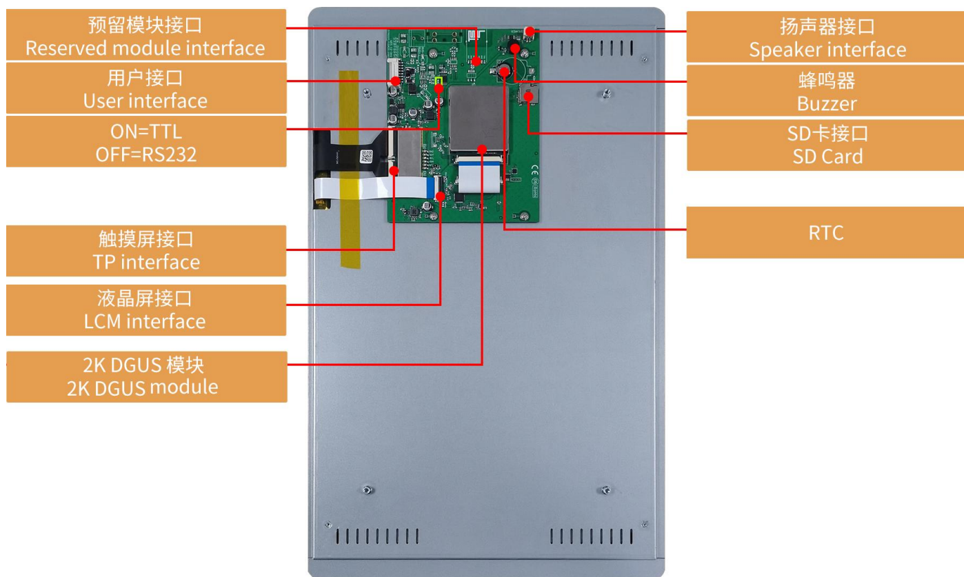
硬件接口图 Hardware interface diagram
