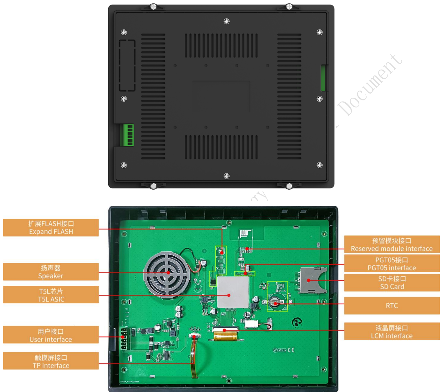
硬件接口图 Hardware interface
